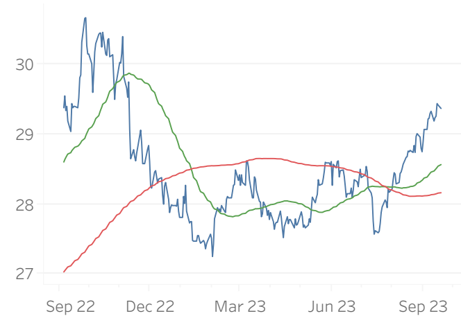
Currencies (UUP)
